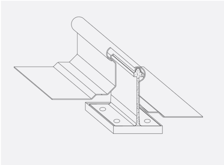
Clips and Motorize Zipper
